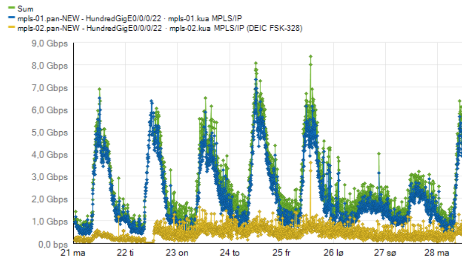
Interface Aggregate Chart - Average bps In Last 7 Days
